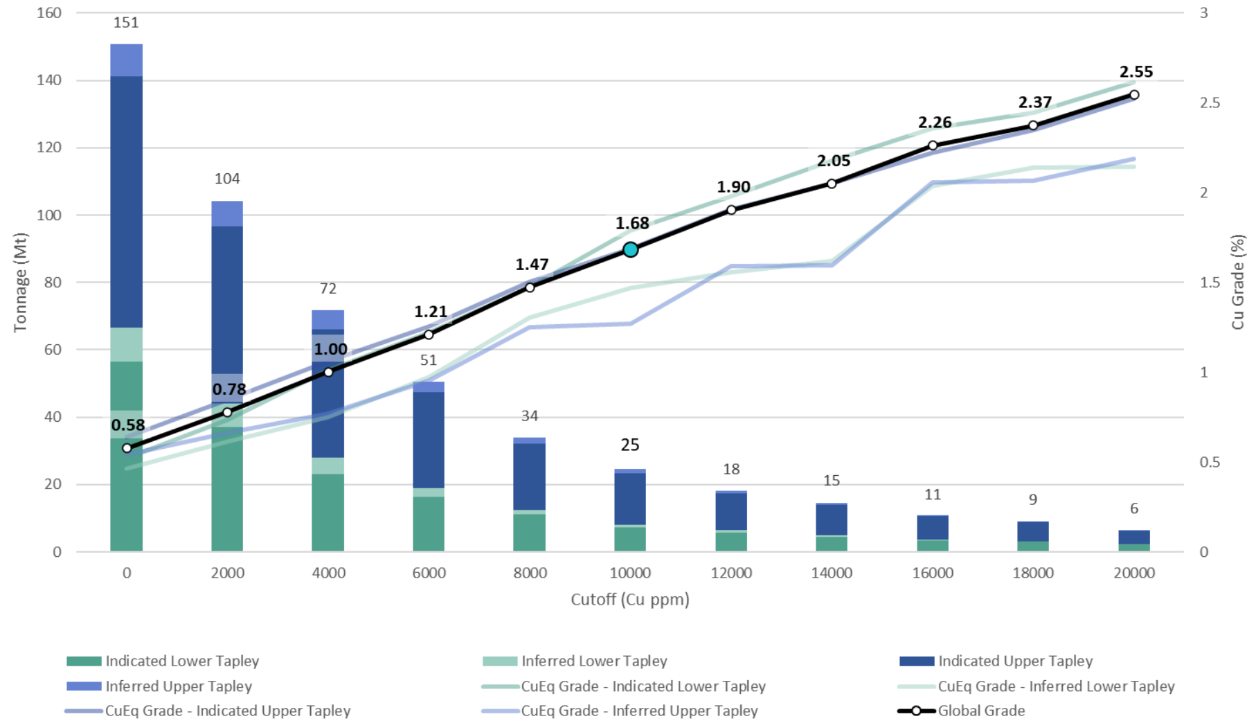
Copper Grade Tonnage Curve (on Cu cut-off grade basis)
