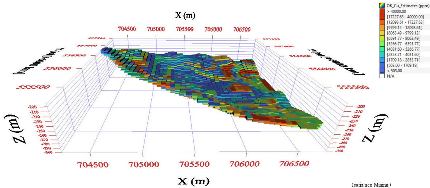
Figure 3 Isometric west view of Emmie Bluff lower Tapley lode (5 times vertical exaggeration).
