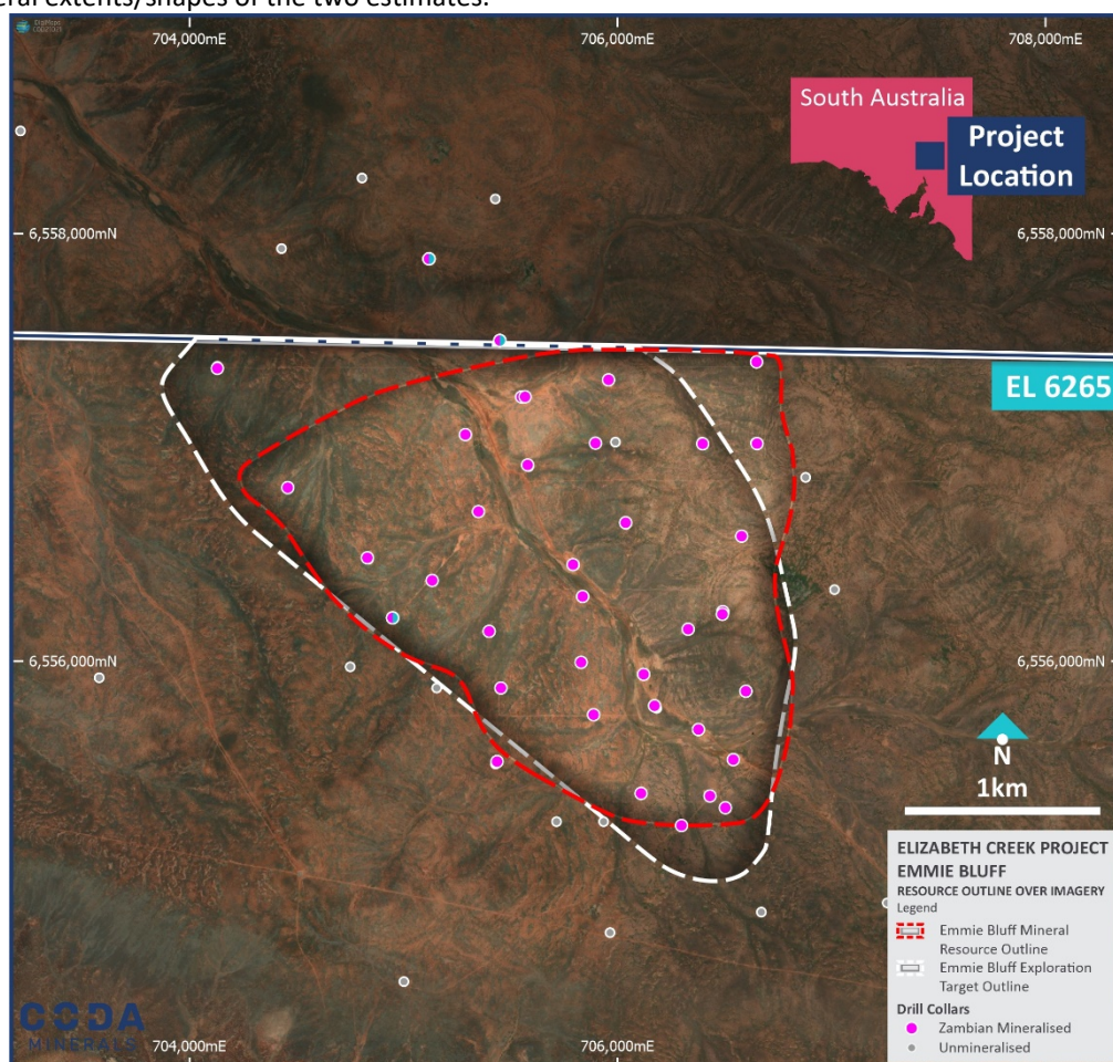
Figure 5 Emmie Bluff Mineral Resource outline (red) overlain over former Emmie Bluff Exploration Target (white) showing differences in geometry and interpreted extent of shale. Some potential exists to extend the mineralisation to the south to test the southernmost tip of the Exploration Target, which currently lacks drill support.
