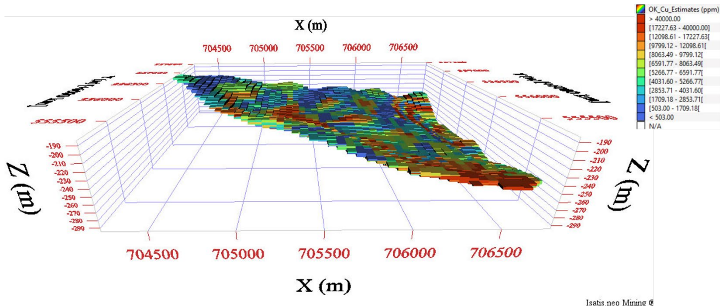
Figure 2 Isometric west view of Emmie Bluff upper Tapley lode (5 times vertical exaggeration).
