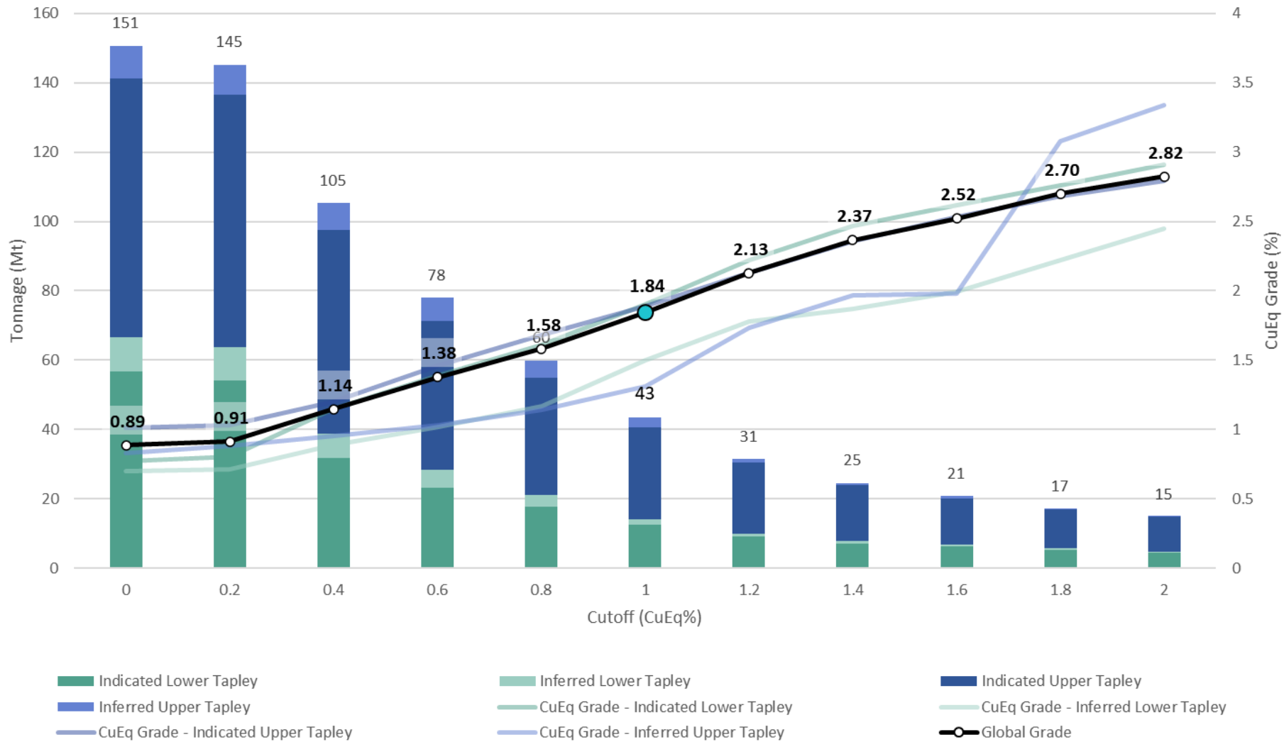
Copper Equivalent Grade Tonnage Curve (on CuEq cut-off grade basis)
