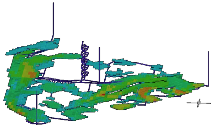
Figure 1. Isometric view of proposed Emmie Bluff slope model.
