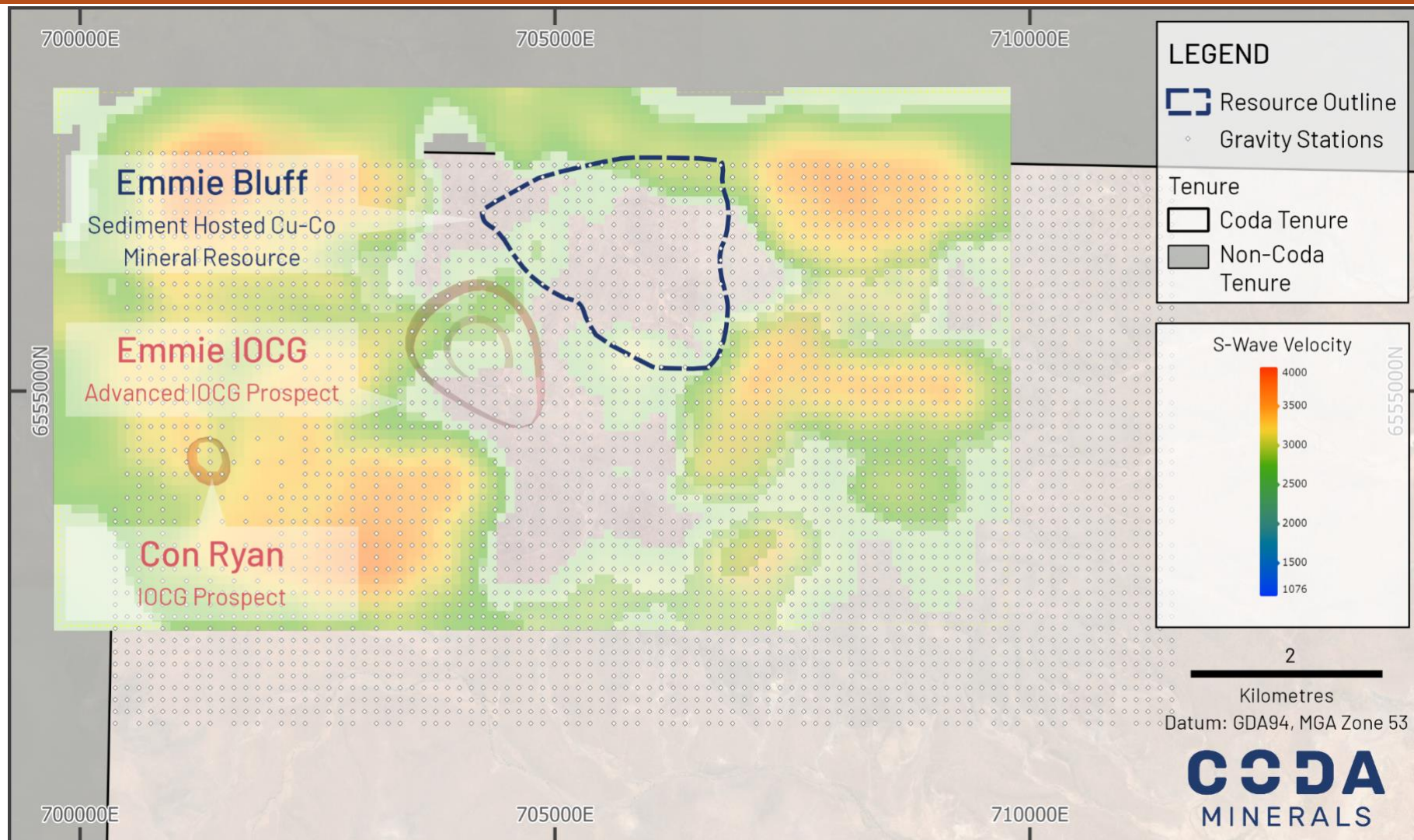
Figure 2 Gravity survey stations overlain on ANT Depth slice and inverted gravity shells at 4.5 g/cc and 4.0 g/cc, -800m RL, 225m slice width. Note the northeast/southwest trending feature associated with the Emmie IOCG gravity anomaly. This will be a priority exploration target going forward.
